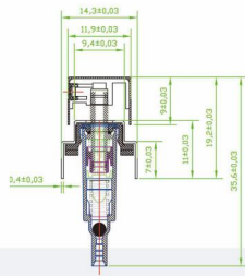
XY-PT-Φ13AB Discharge Rate: 0.06-0.07ml/T
