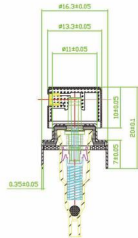
Series: No.1 XY-PT-Φ15/AMG Discharge Rate: 0.09-0.1ml/T No.2 XY-PT-Φ15/AJD Discharge Rate: 0.07-0.08ml/T
