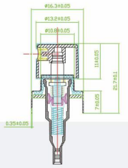
Series: No.1 XY-PT-Φ15MG Discharge Rate: 0.1-0.11ml/T No.2 XY-PT-Φ15JDB Discharge Rate: 0.07-0.08ml/T
